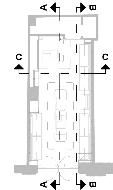
KEY PLAN SCALE 1:150 DIMENSION IN CM
