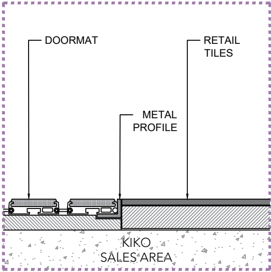
DETAIL 02_FLOORING SCALE 1:5
