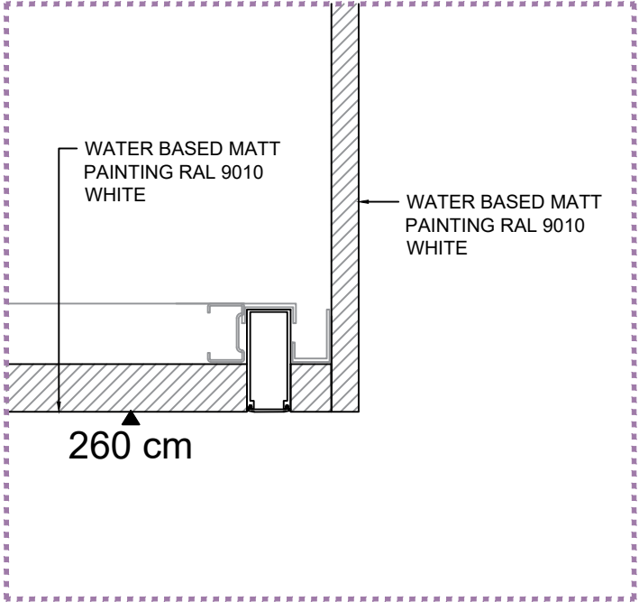
DETAIL 01_Ceiling SCALE 1:5
