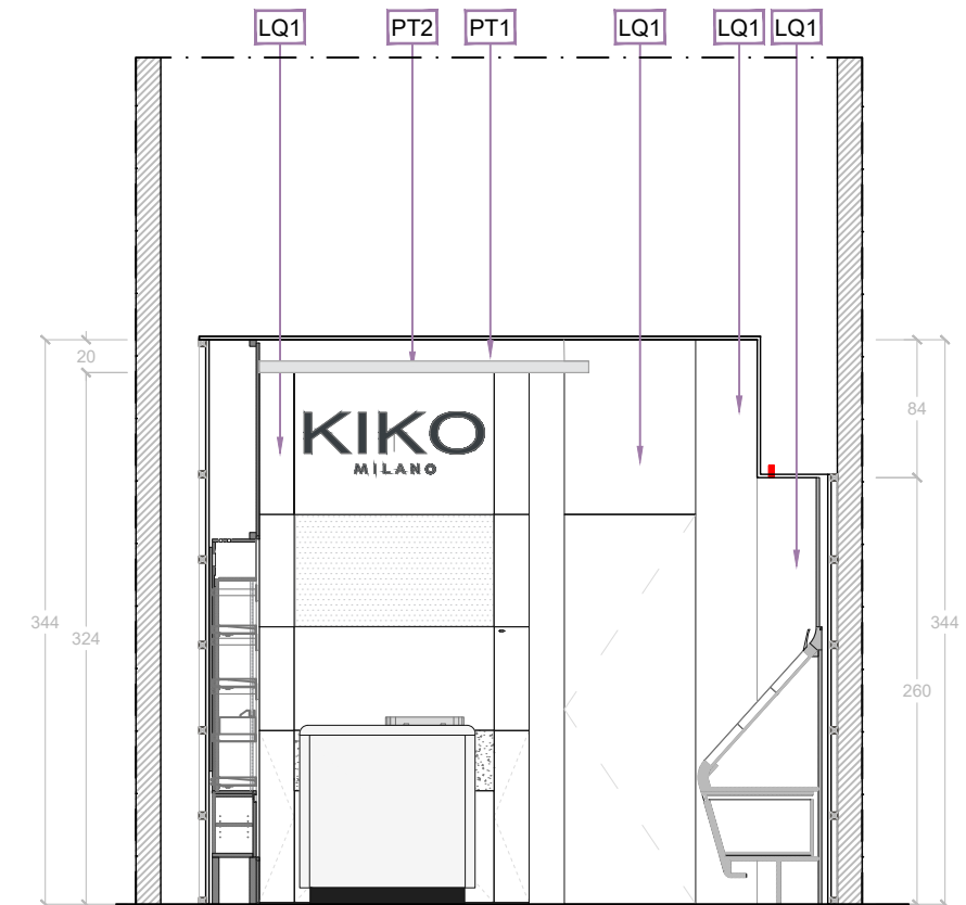
SECTION C-C
