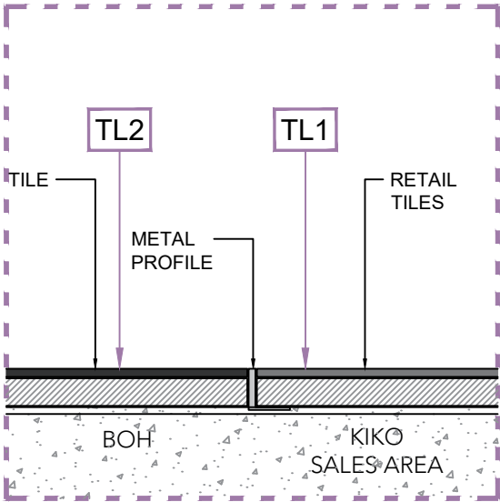
DETAIL 01_FLOORING SCALE 1:5
