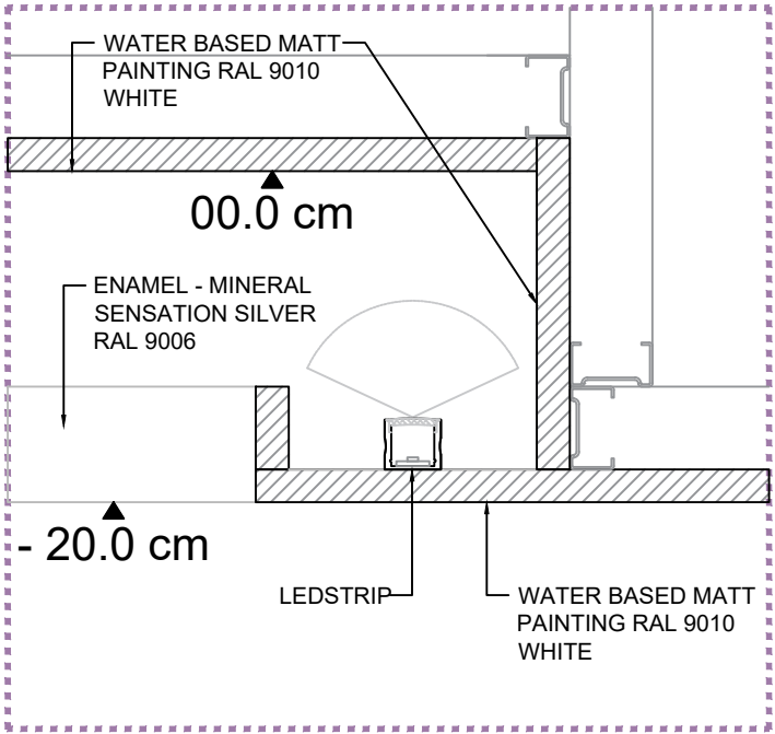
DETAIL 02_Ceiling SCALE 1:5
